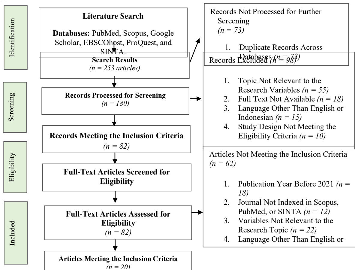
Figure 1. Prisma Flowchart
